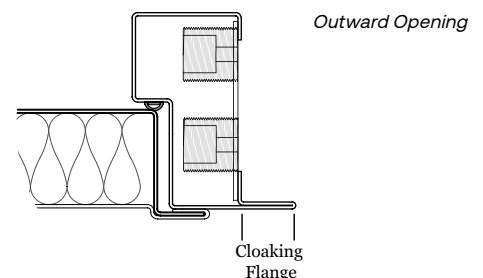
Outward Opening
