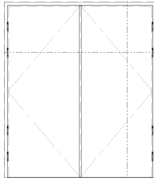
Double Door or Leaf and a Half
